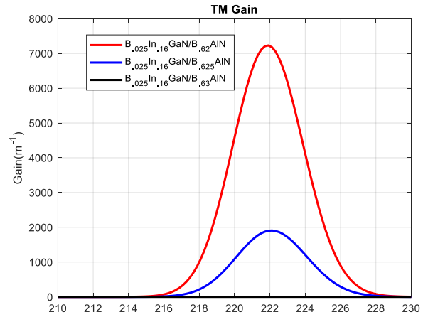
FIGURE 13: THE TE AND TM GAIN MODES AND SPONTANEOUS EMISSION FOR BInGaN/AlGaN QD STRUCTURE.
