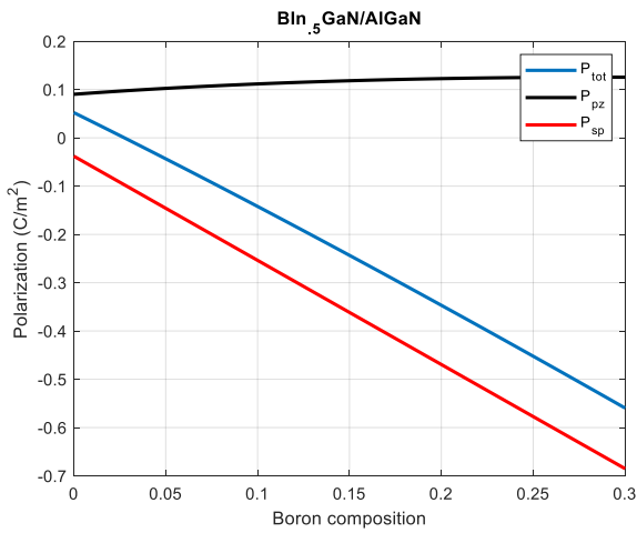
FIGURE 14: THE POLARIZATION COMPONENTS FOR BInGaN/AlGaN QD STRUCTURE.
