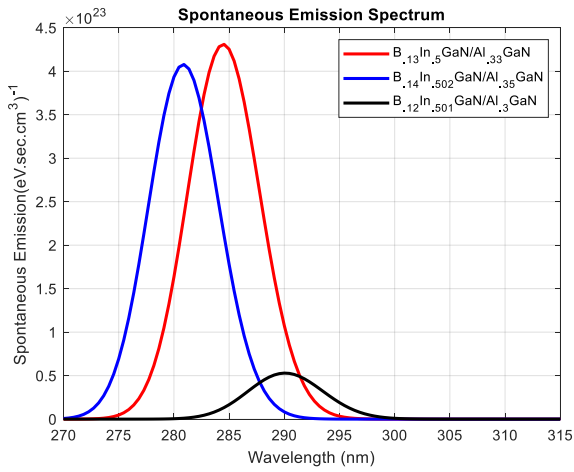
FIGURE 13: THE TE AND TM GAIN MODES AND SPONTANEOUS EMISSION FOR BInGaN/AlGaN QD STRUCTURE.
