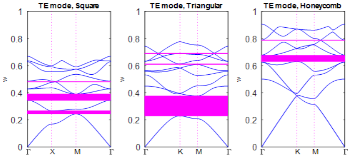
Fig. 6: Band structures of TE modes in 2D PhC lattices with radius R=0.38a for the first type.
