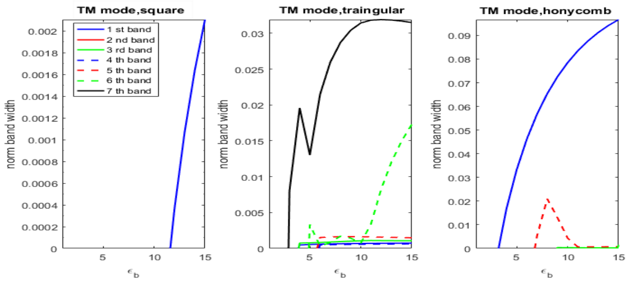
Fig. 3: The normalized band width of TM modes in first type lattice as function of \epsilon_b for R = 0.38a .
