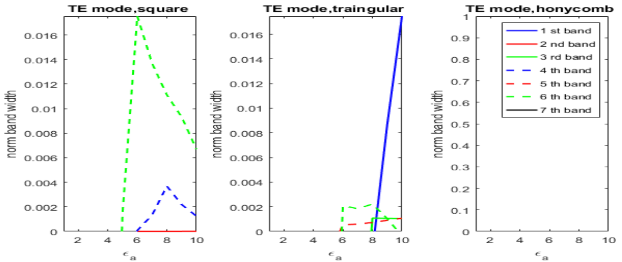
Fig. 4: The normalized band width of TE modes in second type lattice as function of \epsilon_a for R = 0.38a .
