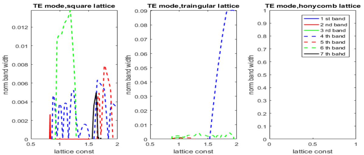
Fig. 7: The norm band width as a function of lattice constant for R = 0.38a of TE modes in second type lattice.
