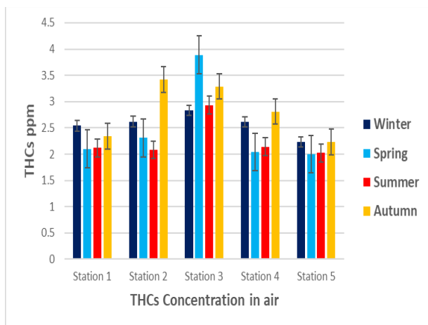
Figure 2. THC concentrations in air (ppm) for four seasons in five selected stations in Al-Nasiriya City, south of Iraq.
