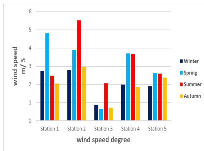
Figure 4. Wind speed in m/s of the selected five stations in Al-Nasiriya City, southern of Iraq.
