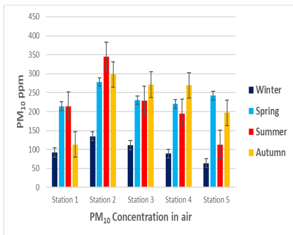
Figure 3. Particulate matter PM 10 concentrations in air (ppm) in the five selected stations among seasons in Al- Nasiriya City, south of Iraq.
