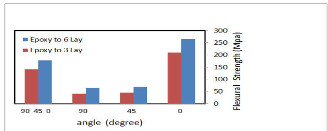
Figure (4): Change the direction of angles with changing flexural strength of epoxy glass fiber samples at (125°C)
