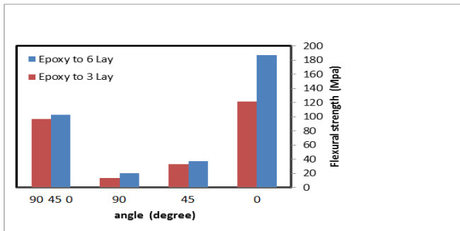
Figure (1): Change the direction of angles with changing flexural strength of epoxy glass fiber samples at (25 °C).
