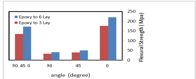
Figure (3): Change the direction of angles with changing flexural strength of epoxy glass fiber samples at (100°C).
