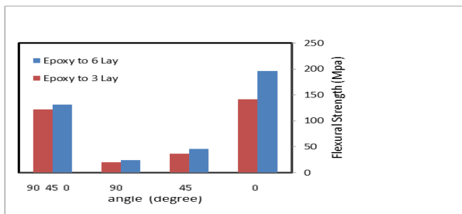
Figure (2): Change the direction of angles with changing flexural strength of epoxy glass fiber samples at (50 ° C).
